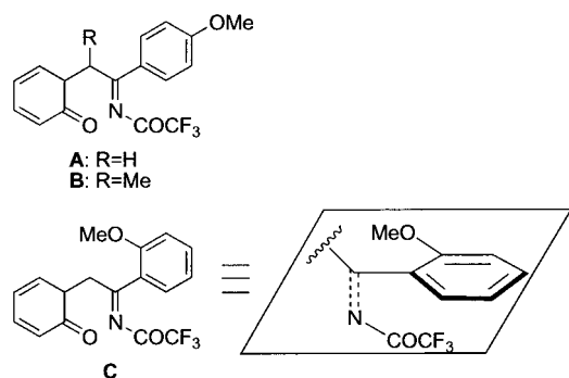
Figure 1. Acylimines A , B , and C with a methoxy group as intermediates.
