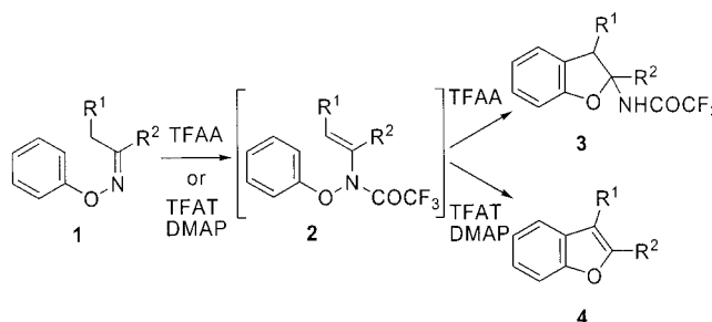
Scheme 1. General reaction of the oxime ethers 1 with TFAA or TFAT-DMAP.
