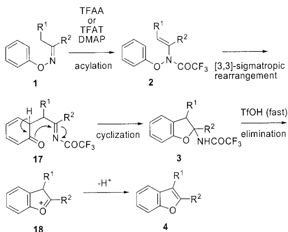
Scheme 2. Possible reaction pathway.
