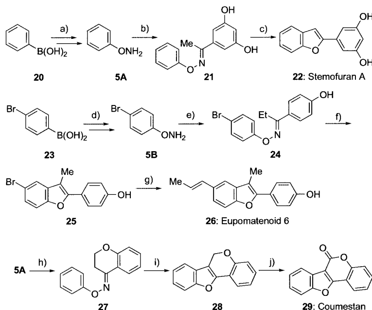
Scheme 3. Short syntheses of Stemofuran A, Eupomatenoid 6, and Coumestan. Reaction conditions: a) 2 steps, 83%, ref. [8] ; b) 3,5-dihydroxyacetophenone, concd. aqueous HCl, EtOH, room temp., 3 h, 92%; c) TFAT, DMAP, CH 2 Cl 2 , room temp., 26 h, 95%; d) 2 steps, 62%, ref. [8] ; e) 4-hydroxypropiophenone, concd. aqueous HCl, EtOH, room temp., 2 h, 92%; f) TFAT, DMAP, CH 2 Cl 2 , room temp., 8.5 h, 95%; g) trans -propenylboronic acid, Pd(PPh 3 ) 4 , CsF, DME, 100 °C, 7 h, 97%; h) 4-chromanone, concd. aqueous HCl, EtOH, room temp., 2 h, 93%; i) TFAT, DMAP, CH 2 Cl 2 , room temp., 4 h, 78%; j) PCC, CH 2 Cl 2 , 40 °C, 4 h, 76%.
